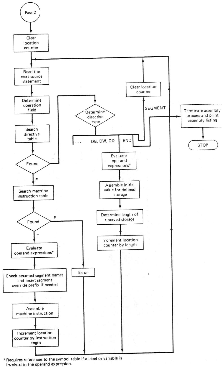
Figure 3-69 Major logic flow of the second pass.
