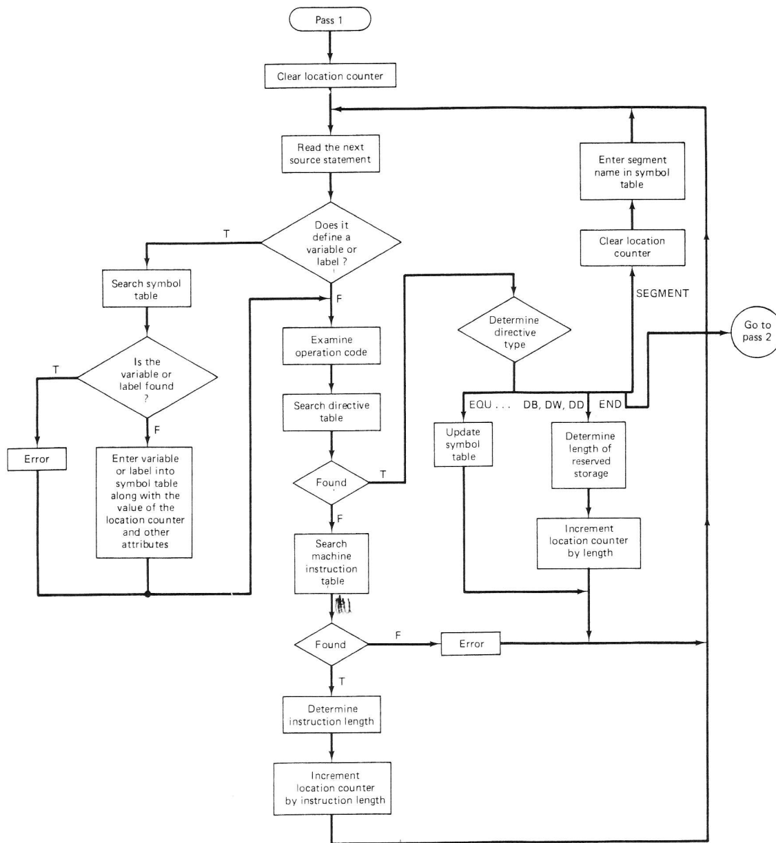
Figure 3-68 Major logic flow of the first pass.
